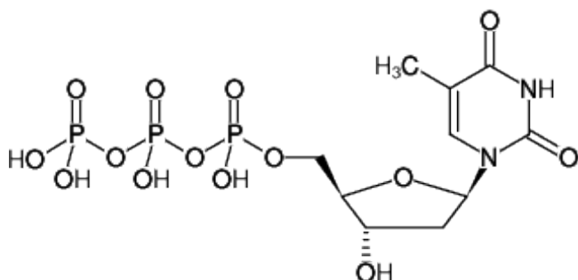
Structural formula of dTTP - Lithium salt solution
