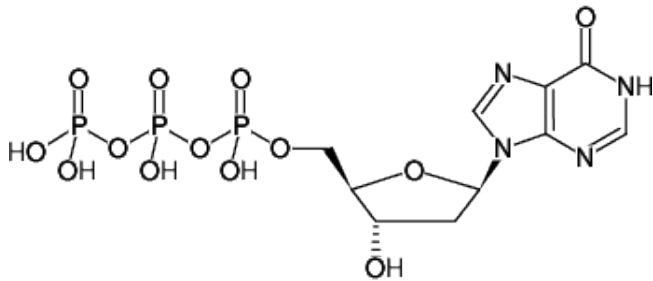
Structural formula of dITP - Sodium salt solution
