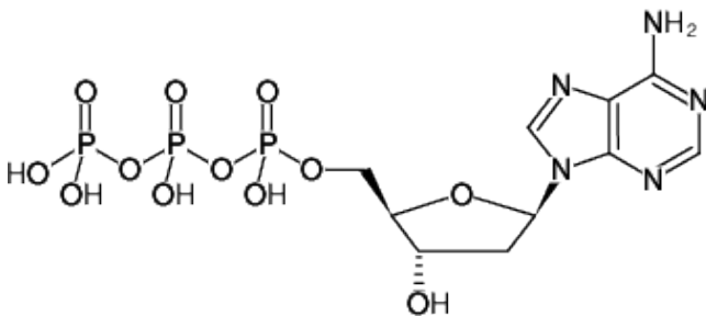
Structural formula of dATP - Lithium salt solution
